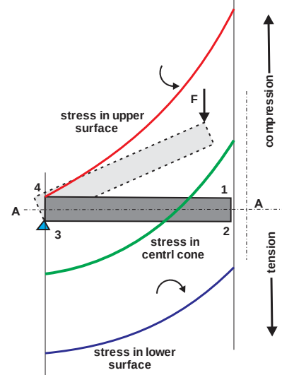
Fig.3. Stress-deflection
